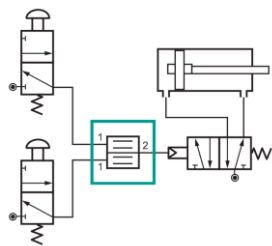
Two-hand safety valve
